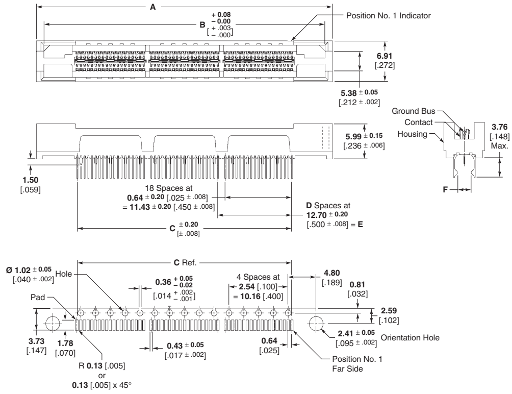
Recommended PC Board Layout (Mirror image on opposite side) PC Board Thickness: 1.57 / [\pm .062]
